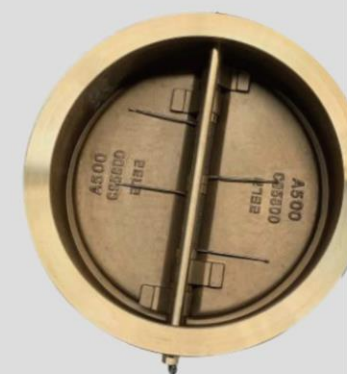
Wafer Check Valve
